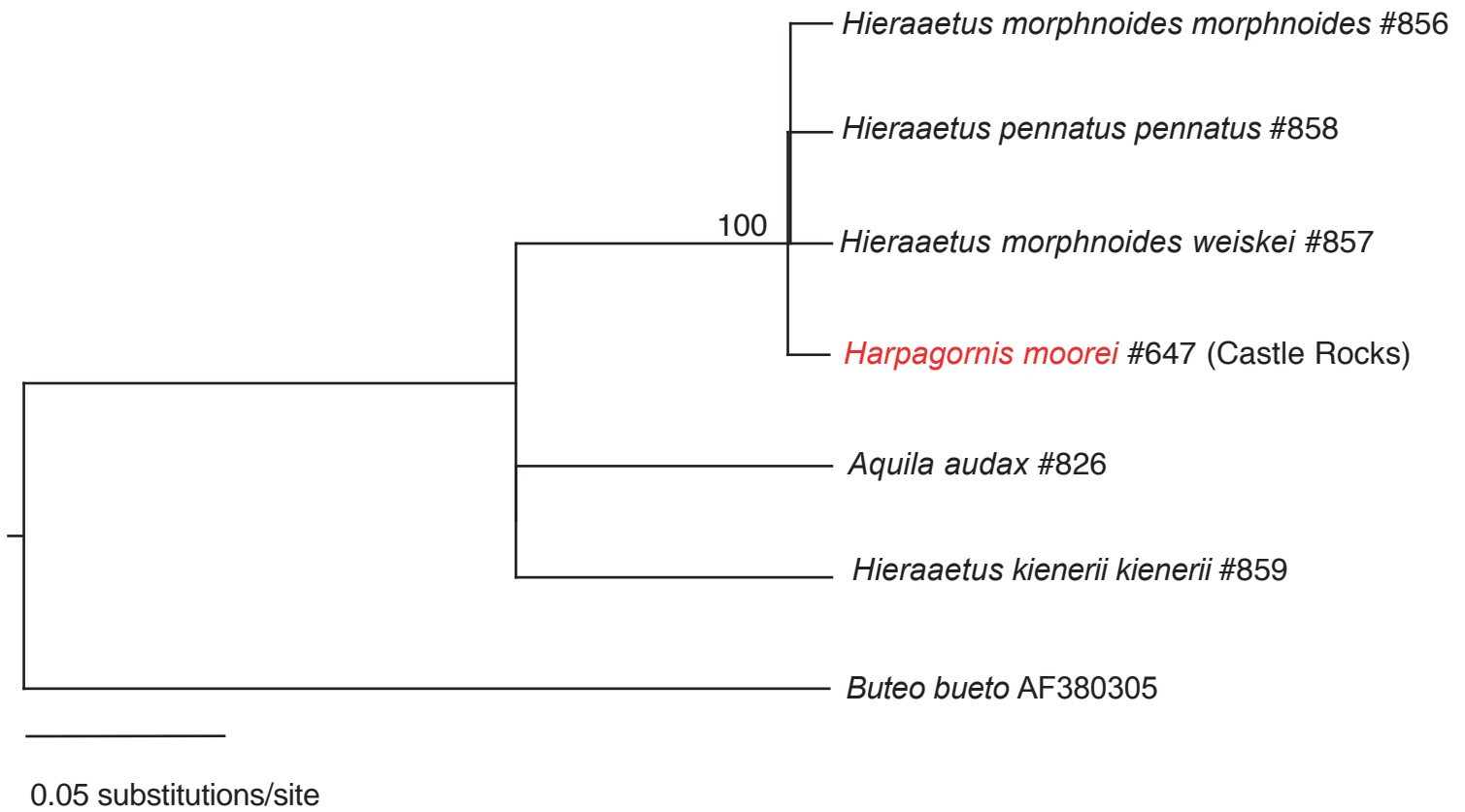
Figure S1. Maximum likelihood tree generated using 434bp of ND2 data from a subset of eagle taxa. The tree topology seen here is identical to that seen in Figure 1C and is an independent verification of the branching order.
